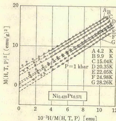
Fig. 4 Arrott plots for Ni_{0.429}Pt_{0.571} 30) .
