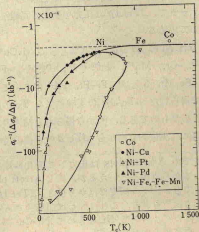
Fig. 7 \sigma_0^{-1} (\Delta \sigma_0 / \Delta p) as a function of T_c for group transition metals and alloys.
