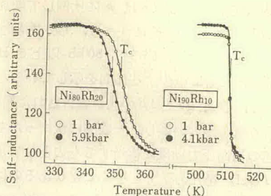
Fig. 3 Self-inductance as a function of temperature at normal pressure and a pressure for Ni_{90}Rh_{10} and Ni_{80}Rh_{20} 18) .
